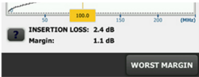
Figure 1. Measured Insertion Loss and limit for 100 foot Type 734 cable.
