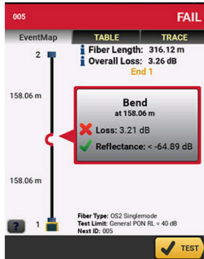
Bend as seen on a EventMap
