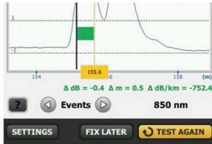
Extremely short event and attenuation dead zone for the Enterprise
