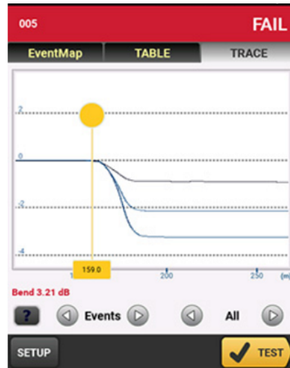
Bend as seen on an OTDR trace
